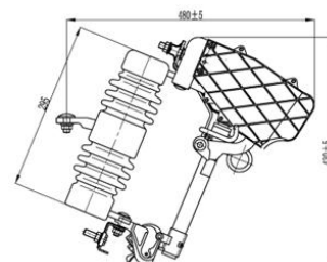
10-15kV Load break Drop-out Fuse
