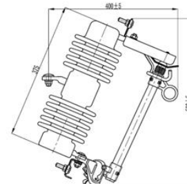
24-27kV Drop-out Fuse
